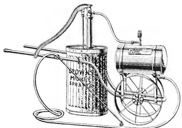
Brown's Mighty Sprayer
